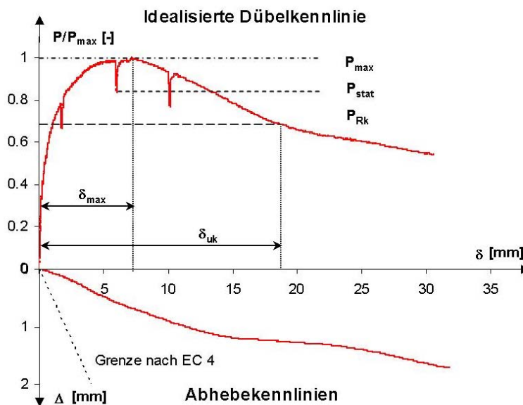
Load-deformation characteristics
